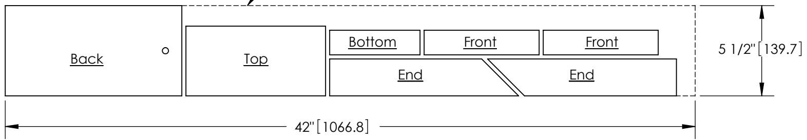
Board Cut Layout
